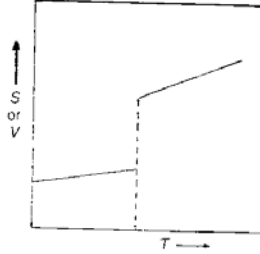
Fig. 4: First order transition showing an idealized phase transition (melting or freezing): Trend of change of volume or entropy with rise of temperature, showing discontinuity at the transition point. (Courtesy: Tata McGraw –Hill, New Delhi)
