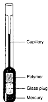
Fig.2: A dilatometric arrangement for measurement of volume change of a polymer with change of temperature.
