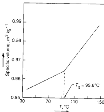
Fig. 3: Temperature dependence of specific volume for polystyrene indicating the glass transition temperature, T_g .
