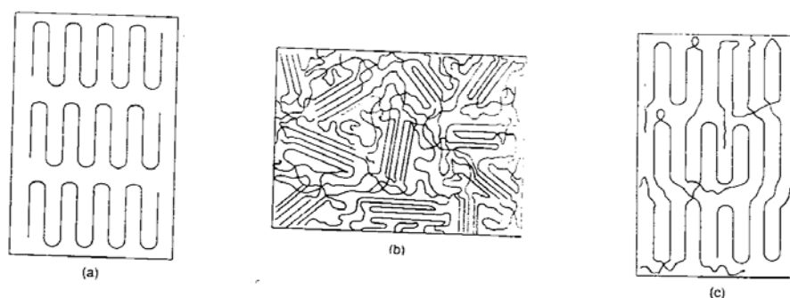
Fig. 17: Schematic representation of (a) ideal stacking of lamellar crystals (discrete folded chains), (b) fringed – micelle model showing randomly distributed amorphous and crystalline zones, and (c) interlamellar amorphous model. (Courtesy: Tata McGraw –Hill, New Delhi)
