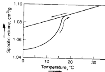
Fig.12: 'Melting curve' showing increase in specific volume ( \text{cm}^3/\text{g} ) vs. temperature ( ^{\circ}\text{C} ) for natural rubber
