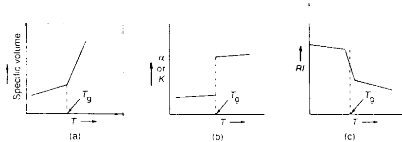
Fig.5: Trends of change in (a) specific volume, (b) coefficient of thermal expansion ( \alpha ) or isothermal compressibility ( K ) and (c) refractive index (RI) of polymers with temperature indicating the glass transition (Courtesy: Tata McGraw- Hill, New Delhi)
