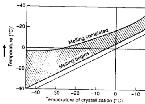
Fig. 14: Plot indicating dependence of melting range of natural rubber on temperature of crystallization, the diagonal line below the melting range (shaded zone) indicating temperature of crystallization. (Courtesy: Tata McGraw –Hill, New Delhi)
